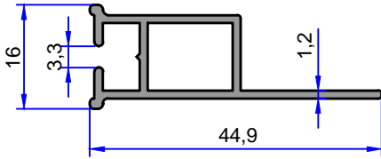
4273 0.325 kg/m
