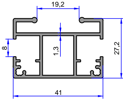
11432 0.668 kg/m
